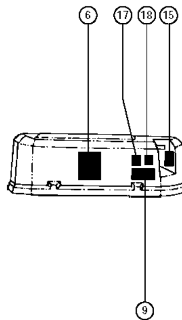
Turntable Cover
